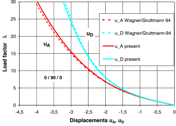
Figure 8: Hyperboloidal composite shell [0^\circ, 90^\circ, 0^\circ] , \lambda - u_A, \lambda - u_D
