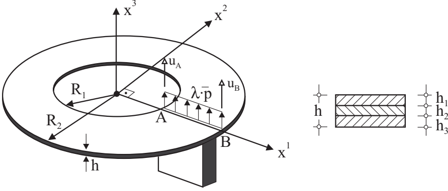
Figure 3: Annular plate
