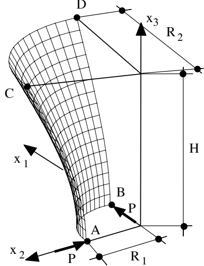
Figure 7: Hyperboloidal composite shell
